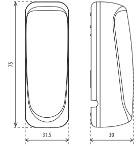
AirWD-100
